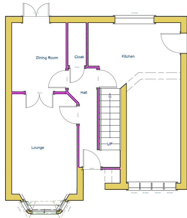
FLOOR PLAN PROPOSED
