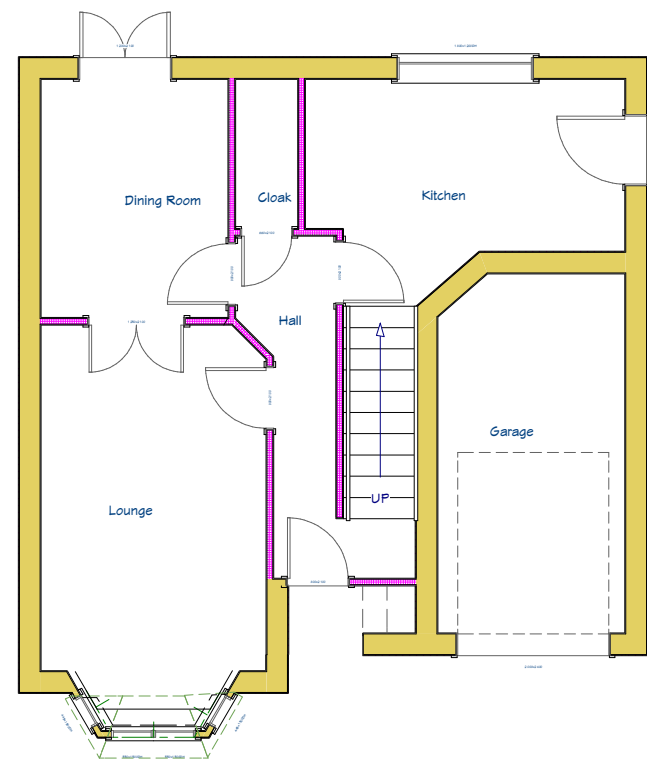
FLOOR PLAN EXISTING
