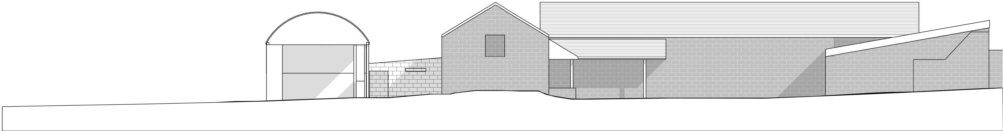
1 East Elevation 1 : 100
