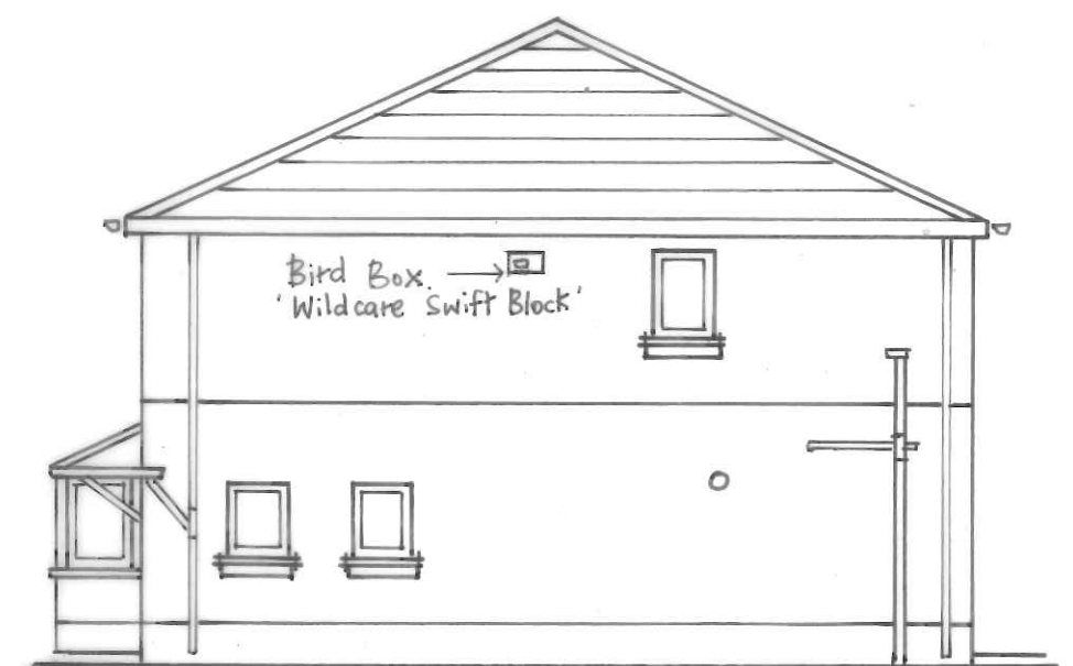
SIDE ELEVATION. [facing sports ground.]
