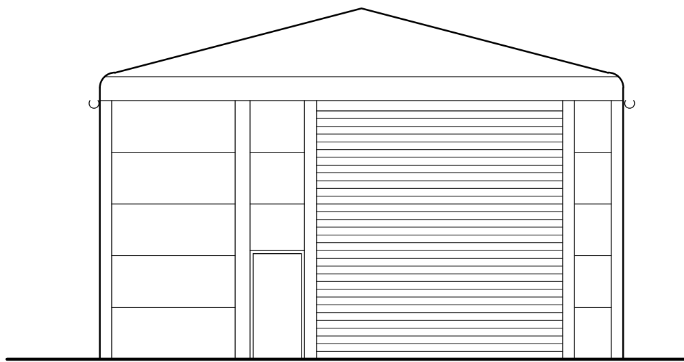
Front Elevation (North)
