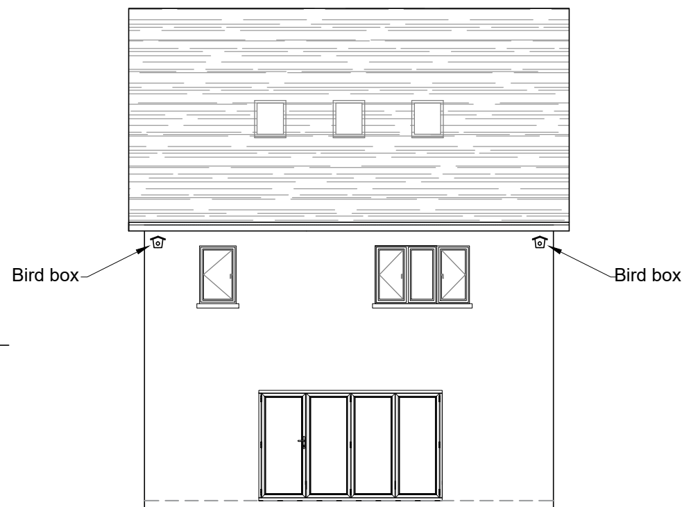
Proposed Rear Elevation (Plot 1) Mirror image for Plot 2 Scale - 1:100
