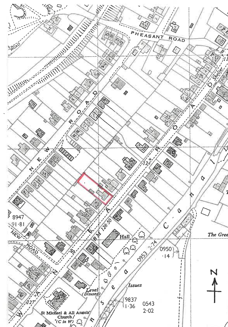
BLOCK PLAN 1:500
