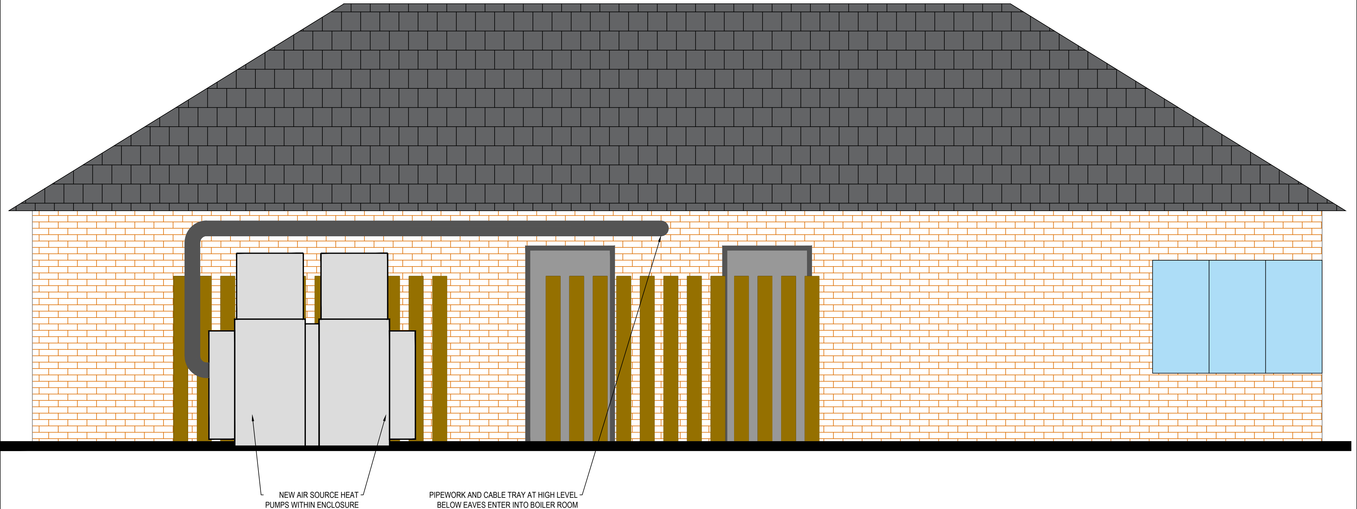
PROPOSED ELEVATION
