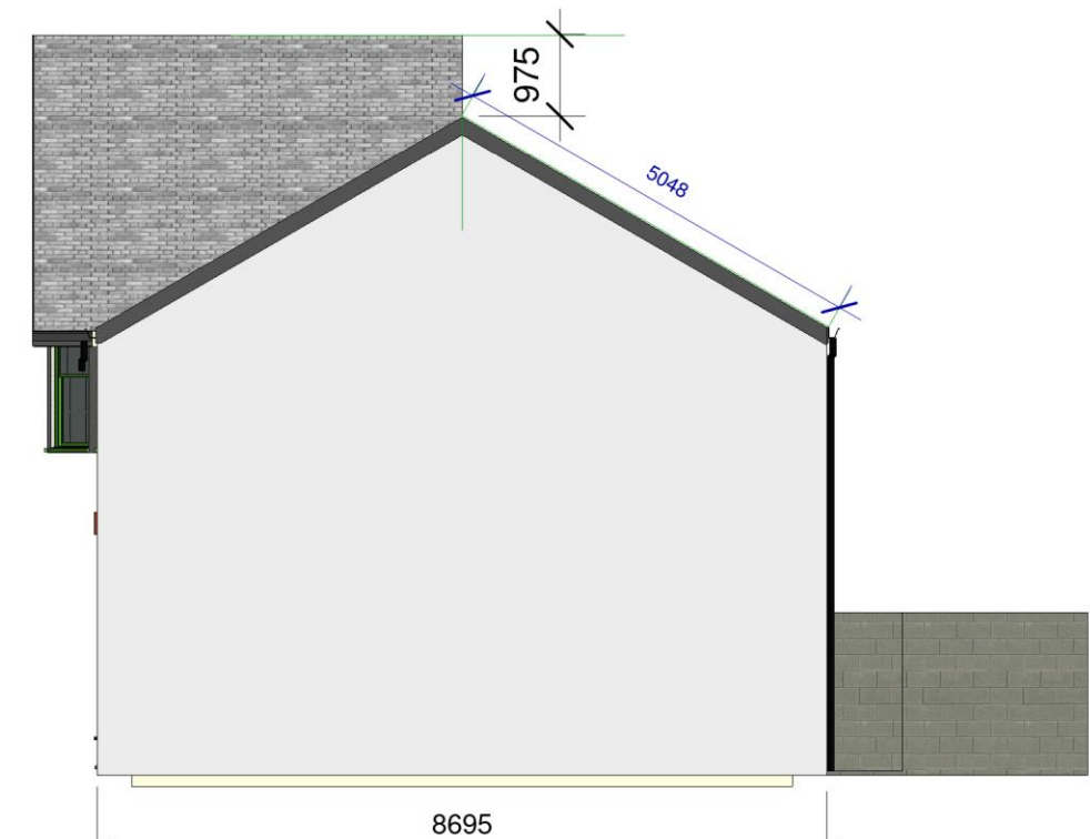
Existing RH Side elevation
