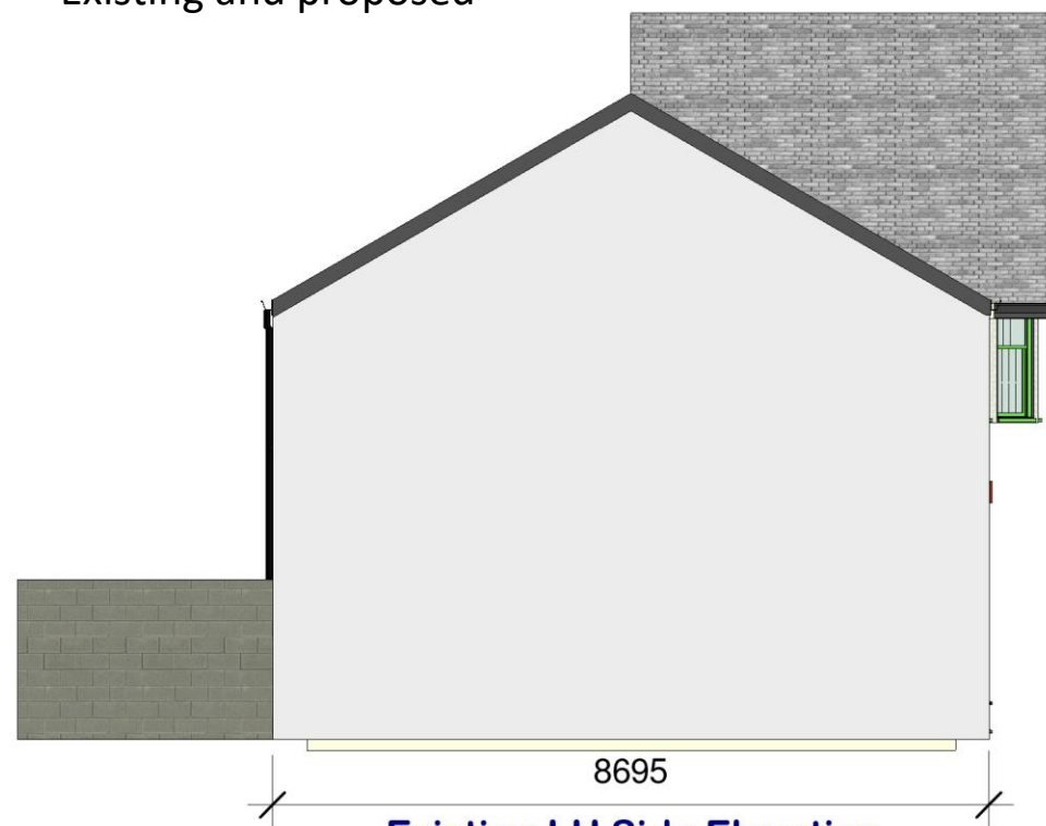
Existing LH Side Elevation
