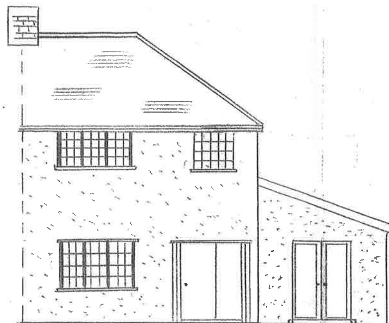
FRONT ELEVATION PROPOSED
