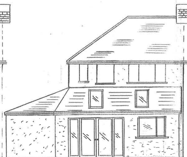
REAR ELEVATION PROPOSED
