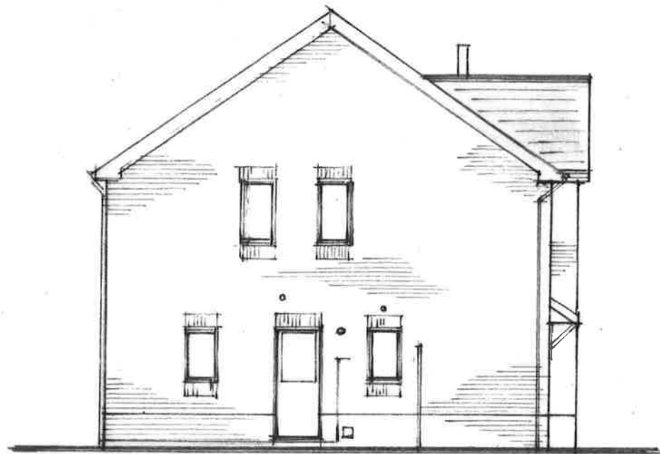
Existing Side Elevation (1:100) (West)
