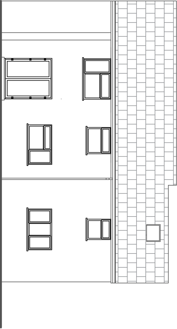
Rear (West) Elevation
