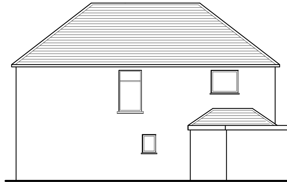
proposed RH Side elevation
