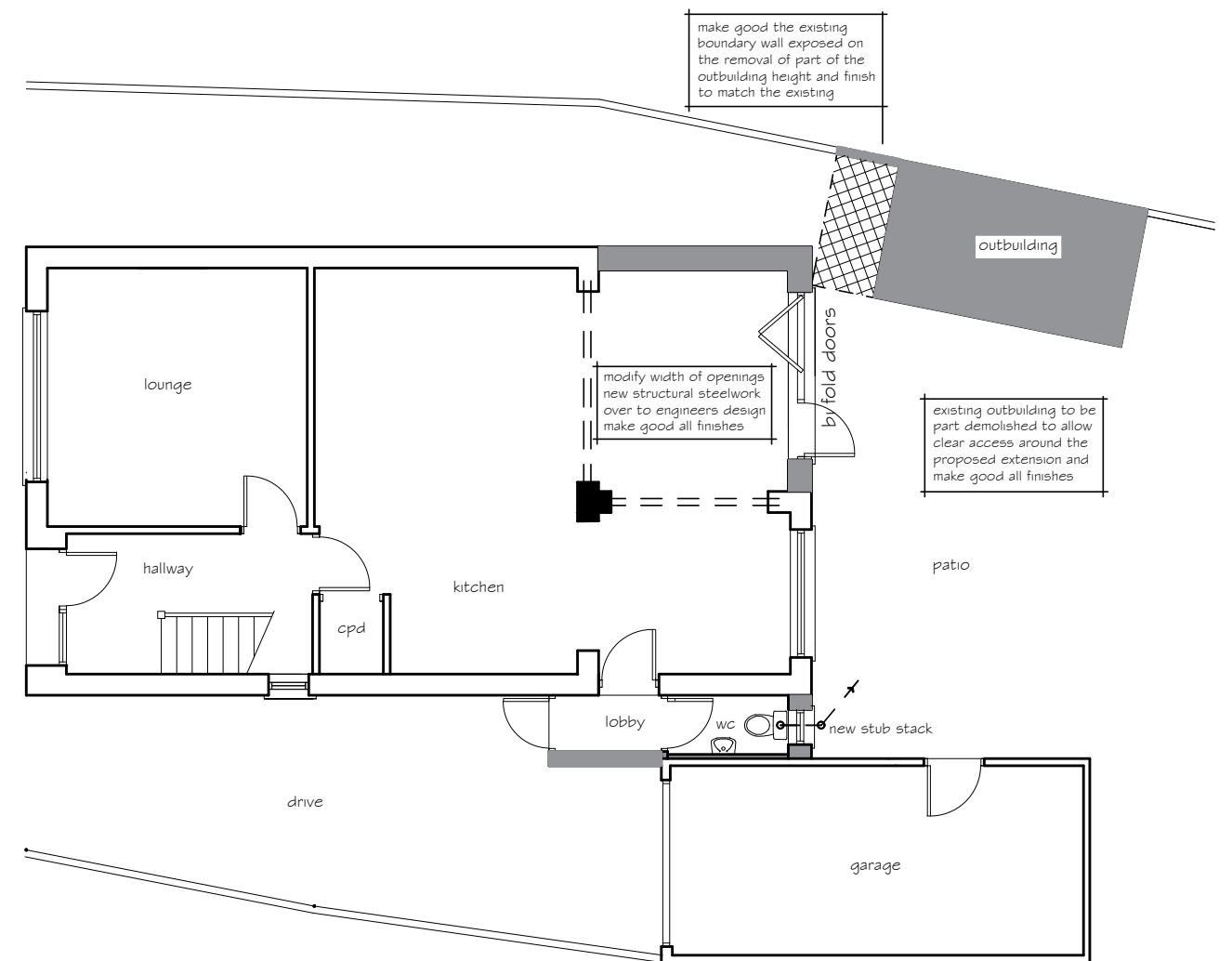
proposed part site plan
