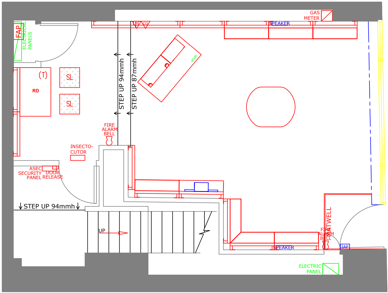
1 Proposed Ground Floor GA Plan Scale: 1:50
