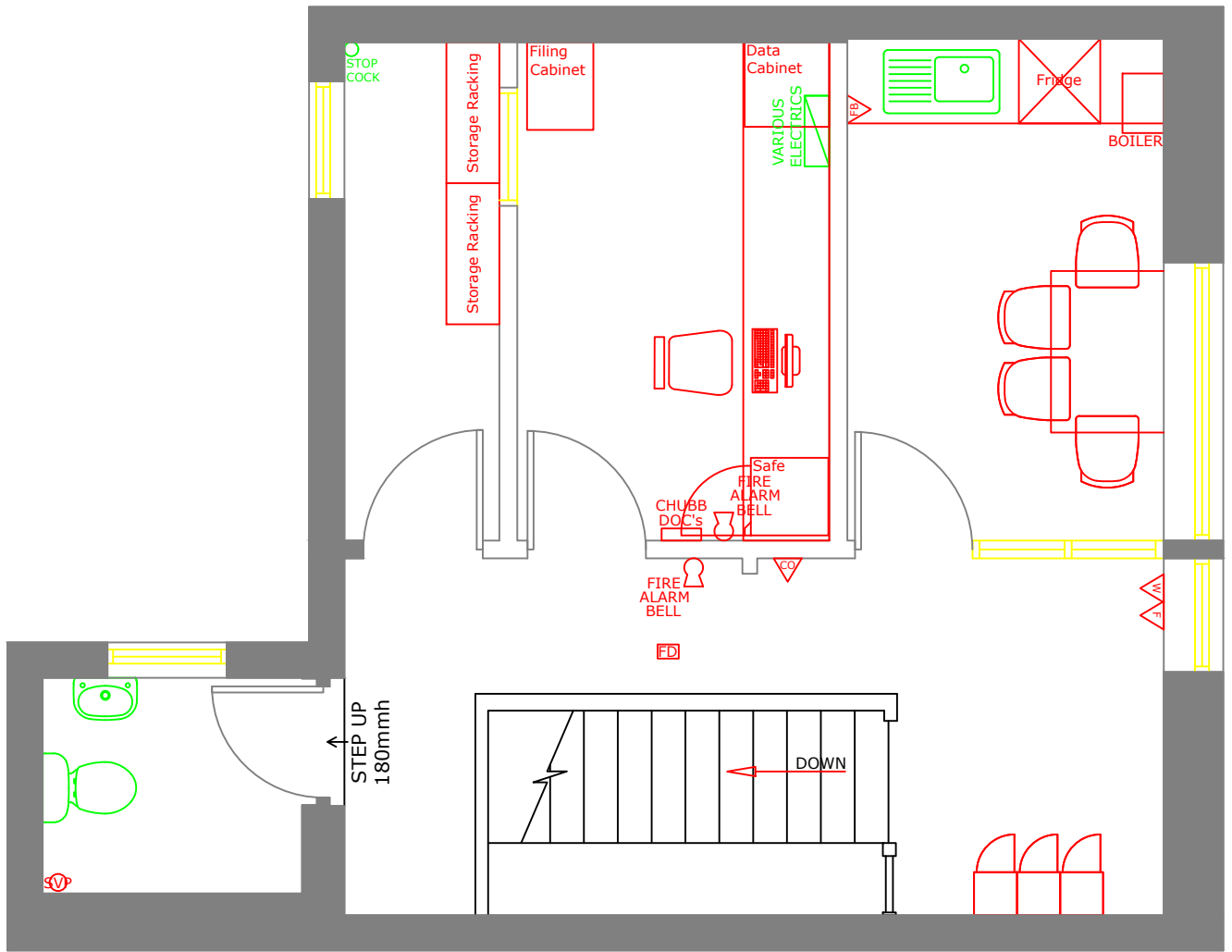
2 Proposed First Floor GA Plan Scale: 1:50
