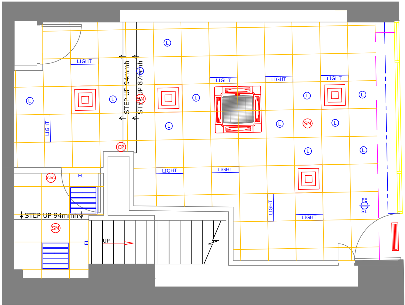
3 Proposed Ground Floor RCP Plan Scale: 1:50
