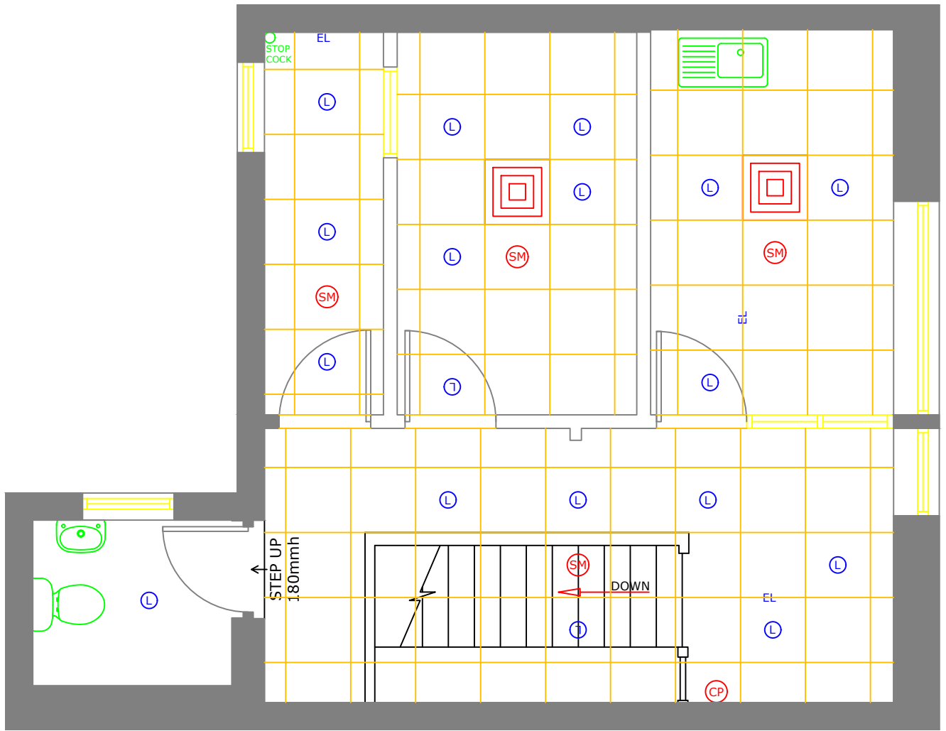
4 Proposed First Floor RCP Plan Scale: 1:50
