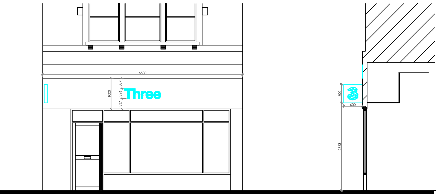
5 Proposed External Elevations Scale: 1:75
