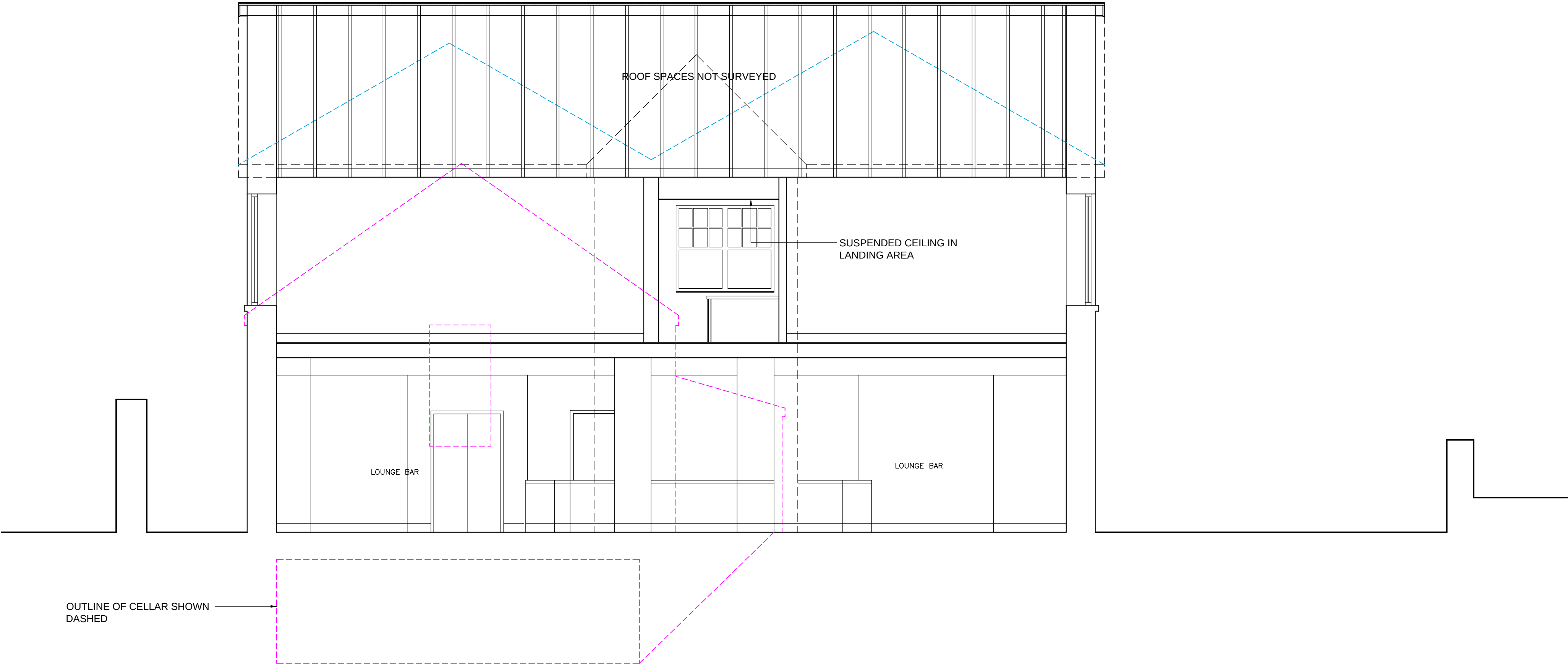
SECTION B-B
