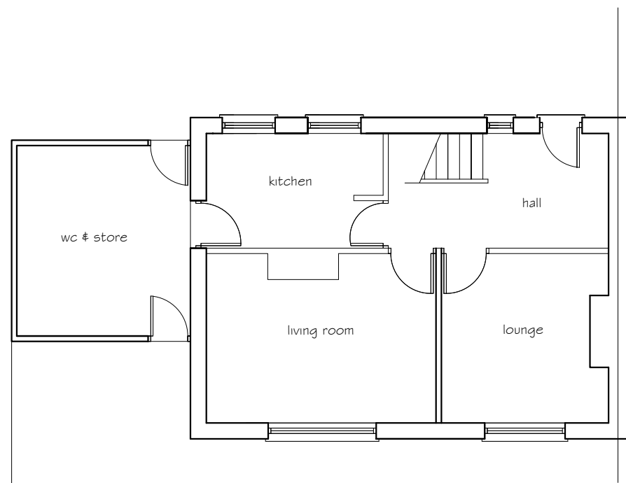
Original ground floor plan
