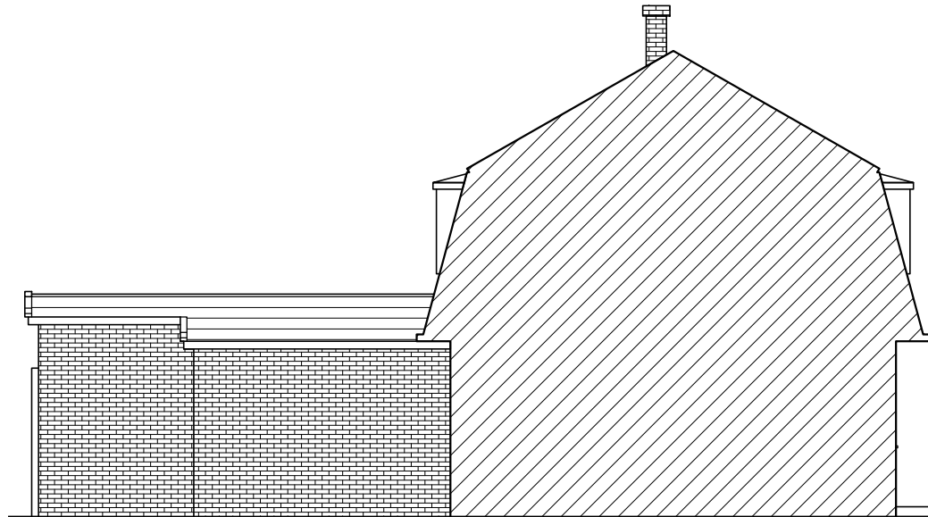
A PROPOSED LEFT SIDE ELEVATION 04 02 SCALE 1:100 M
