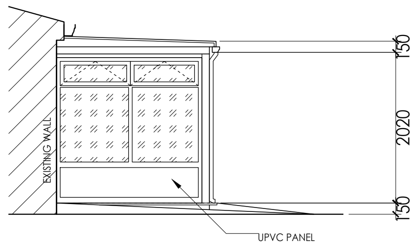
CONSERVATORY LEFT SIDE ELEVATION
