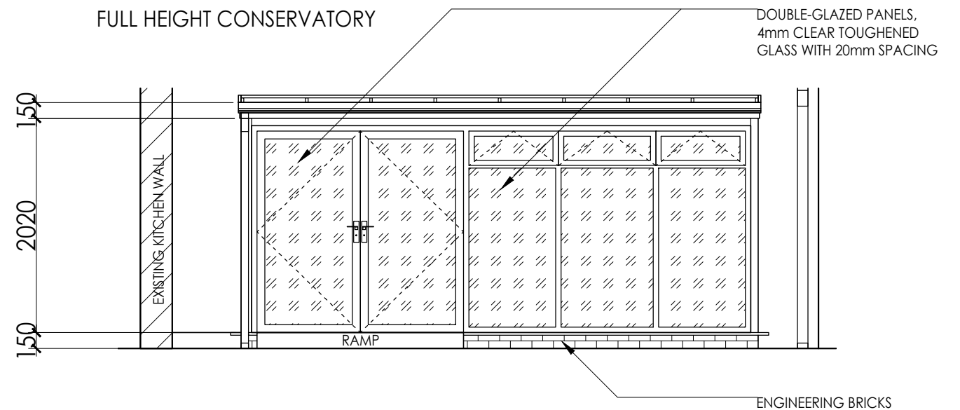
CONSERVATORY FRONT ELEVATION
