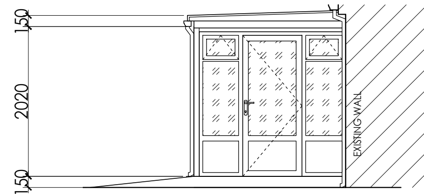
CONSERVATORY RIGHT SIDE ELEVATION
