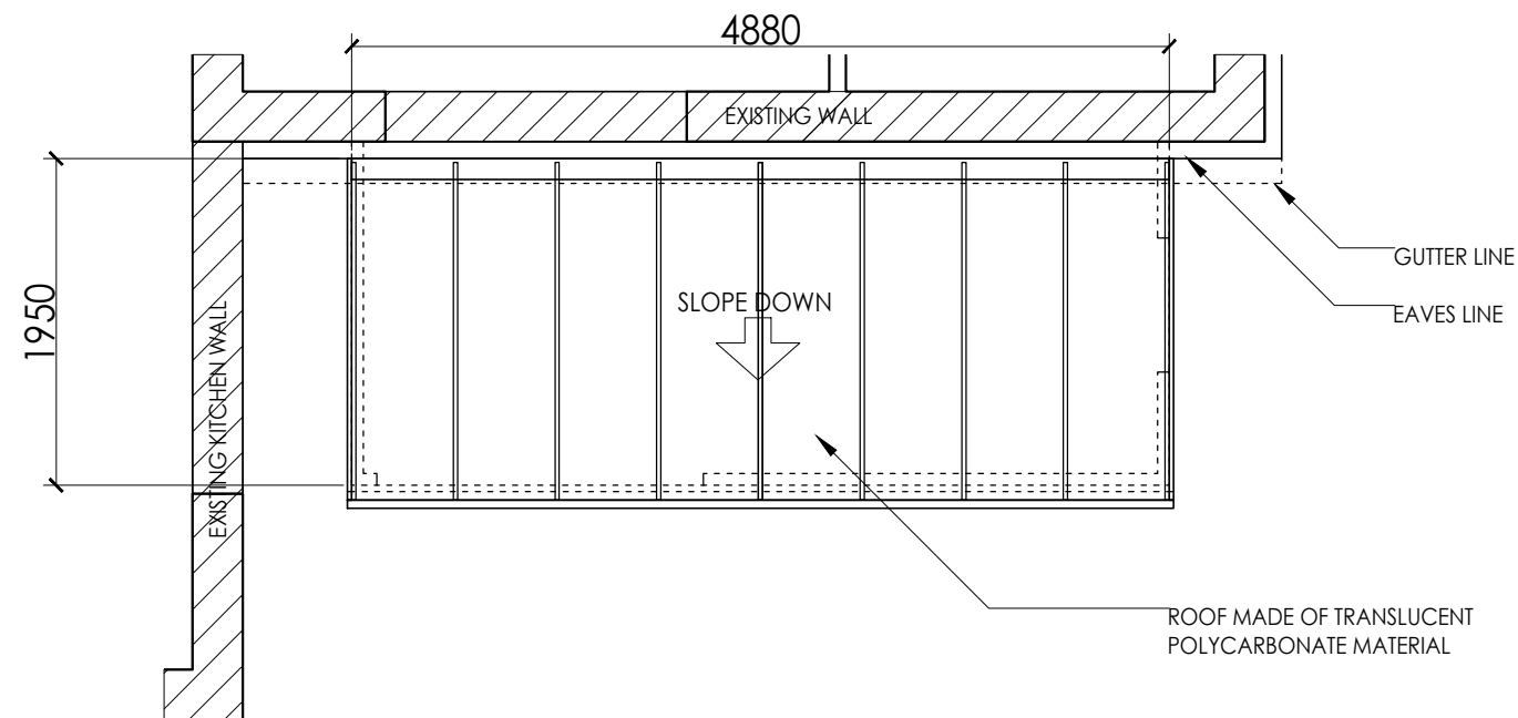
CONSERVATORY ROOF PLAN
