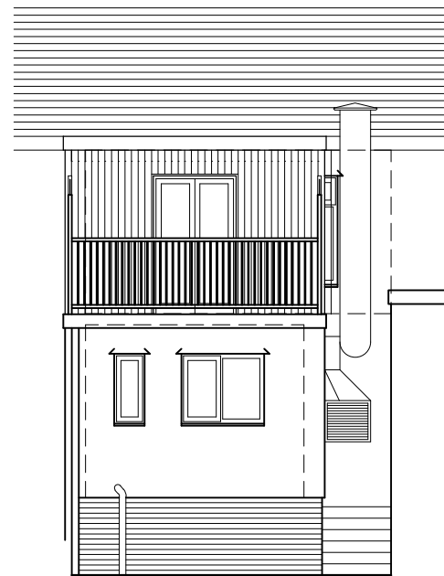
Rear (north) elevation 1:100
