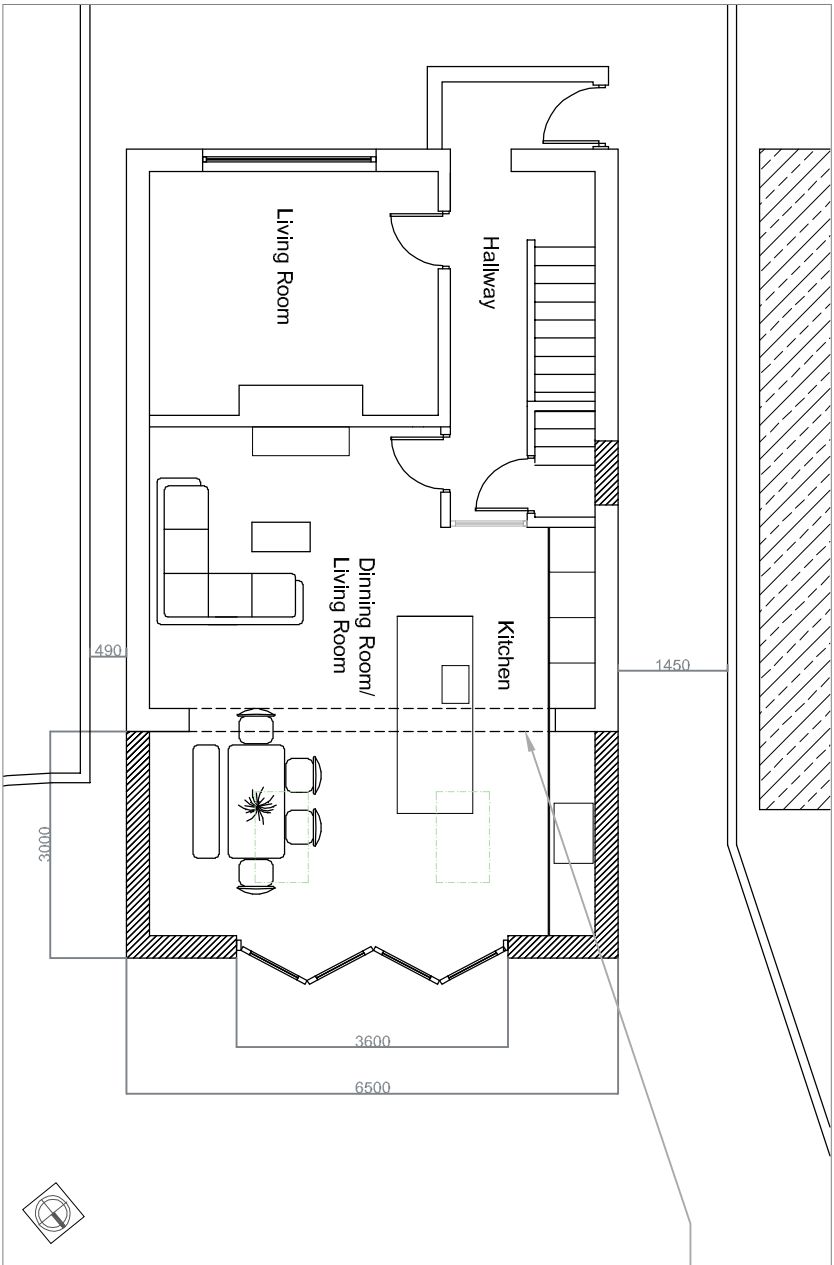
Plan Scale 1:100
