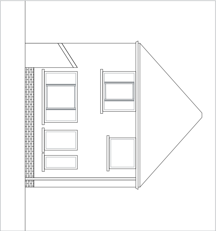
North Elevation Scale 1:100
