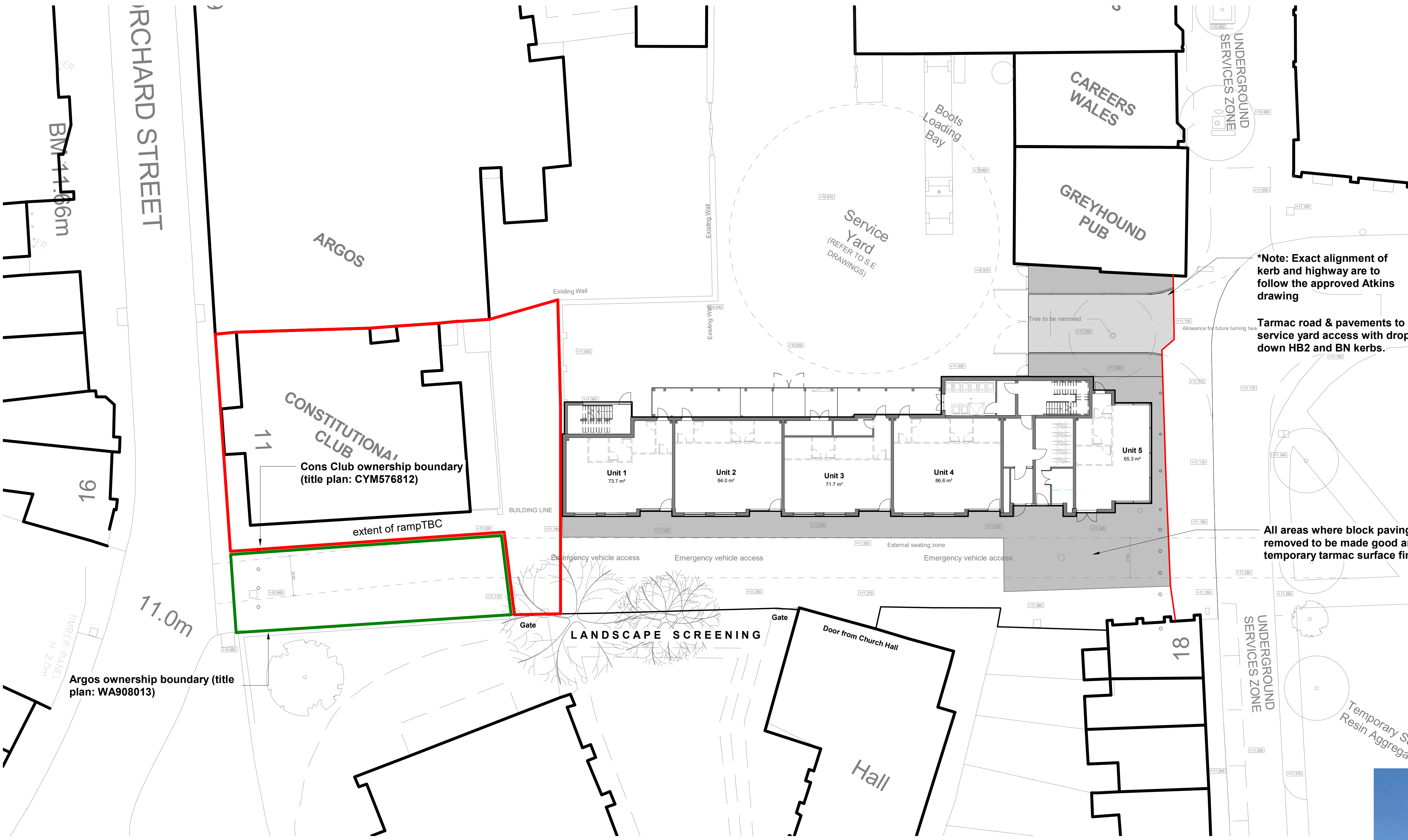
External Works _Extent of Lane _Temp Finish 1 : 200
