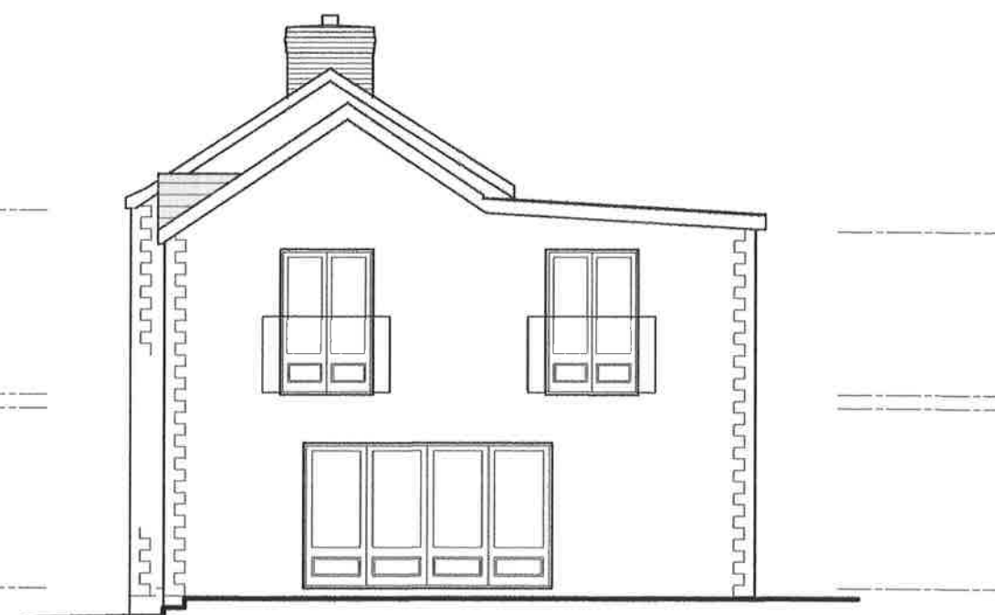
NORTH-WEST ELEVATION
