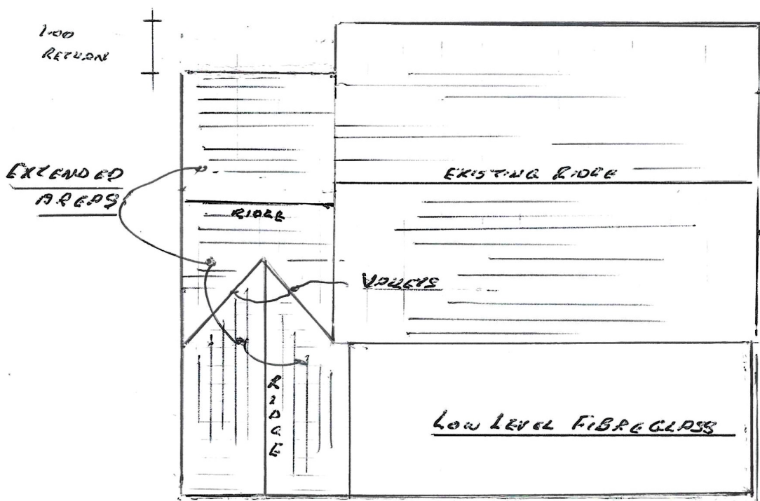
SCALE 1:100 PROPOSED ROOF PLAN
