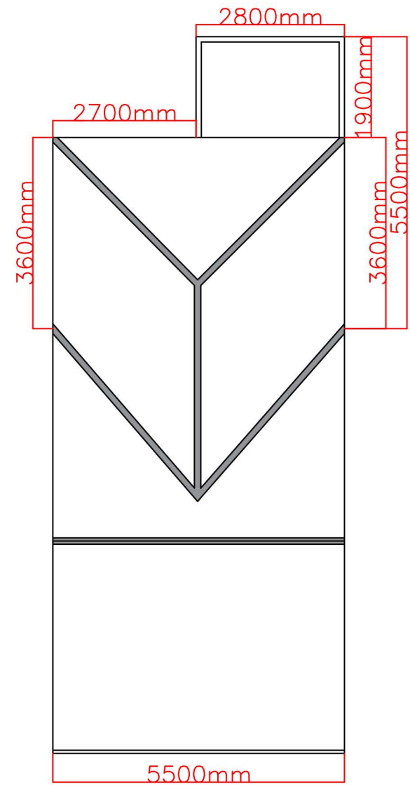
Birdseye View
