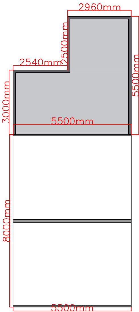
Current Top Down View
