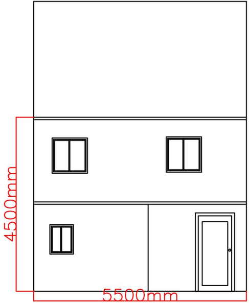
Current Rear Elevation View
