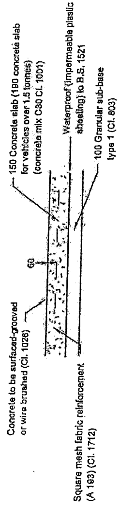
STANDARD CONSTRUCTION IN VEHICLE CROSSINGS TYPE FC3
