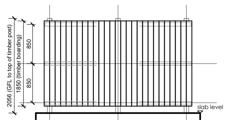
Side Elevation(s)
