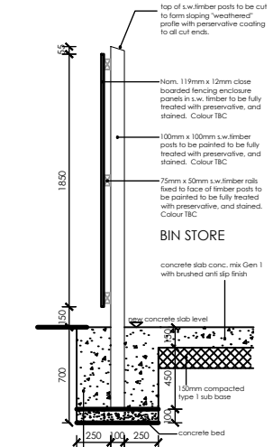
Typical Section
