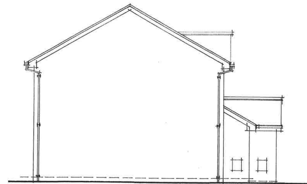
SIDE ELEVATION
