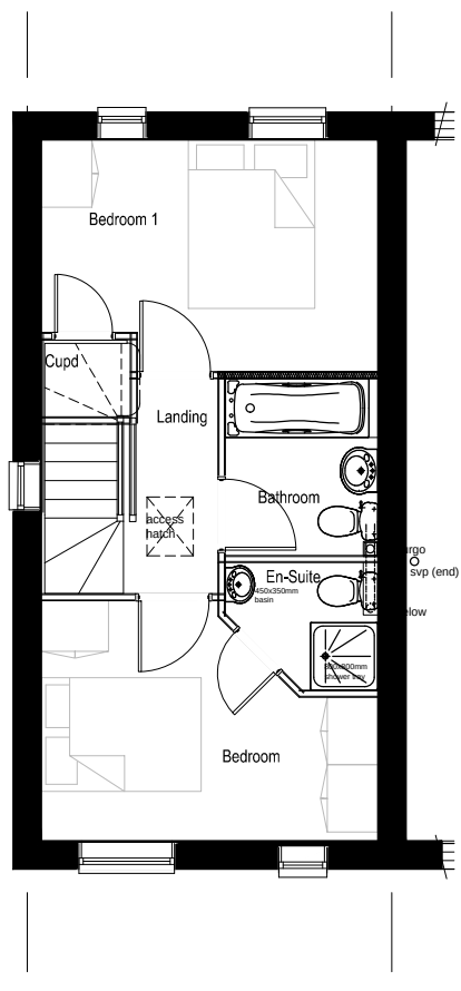
Second Floor
