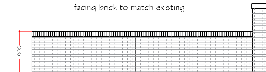
Proposed boundary wall 1:100
