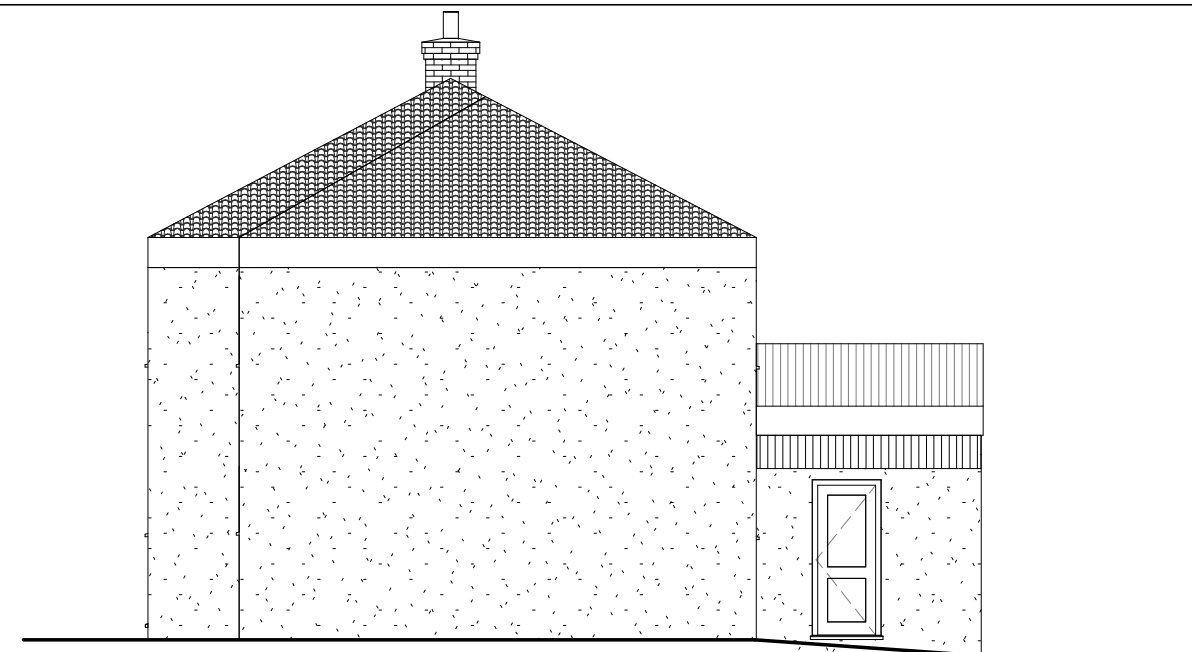
Existing Right Elevation
