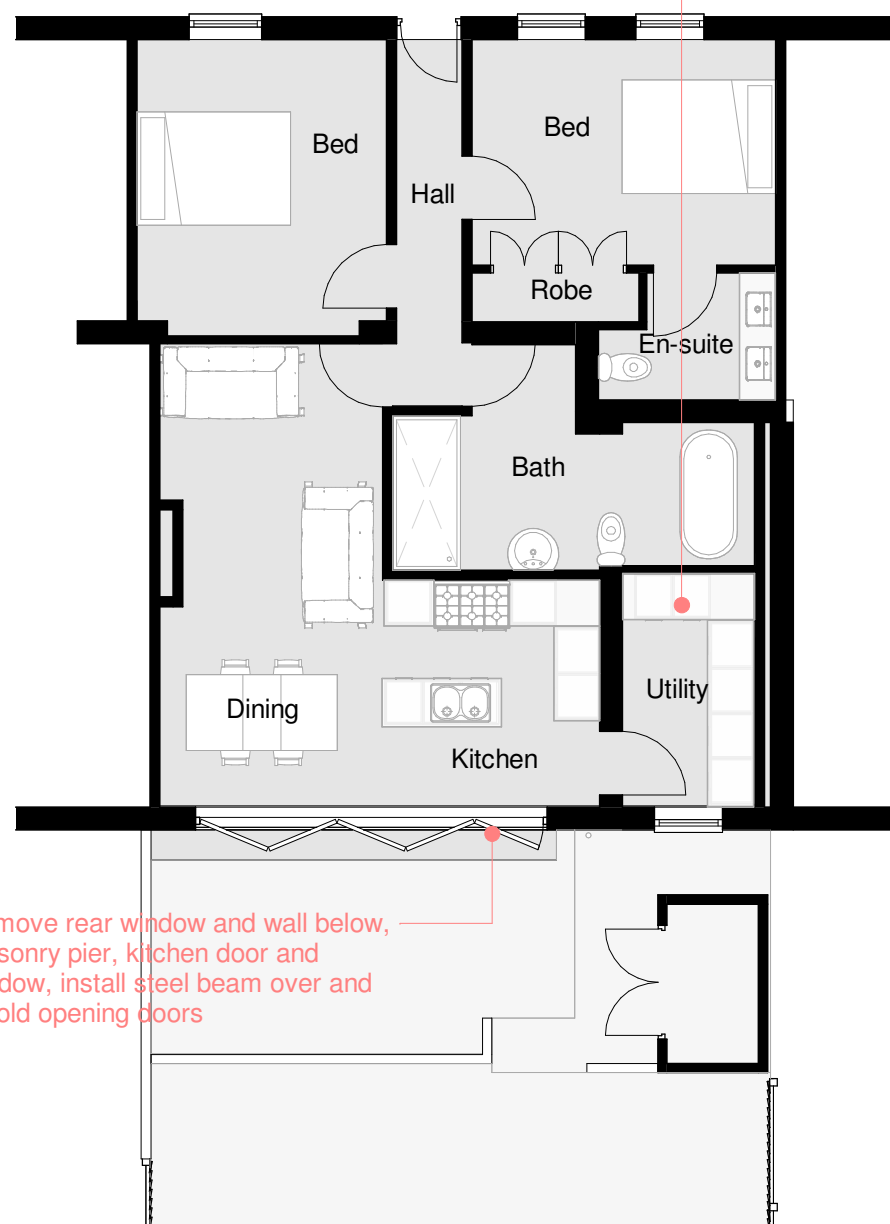
PROPOSED FLOOR PLAN 1 : 100
