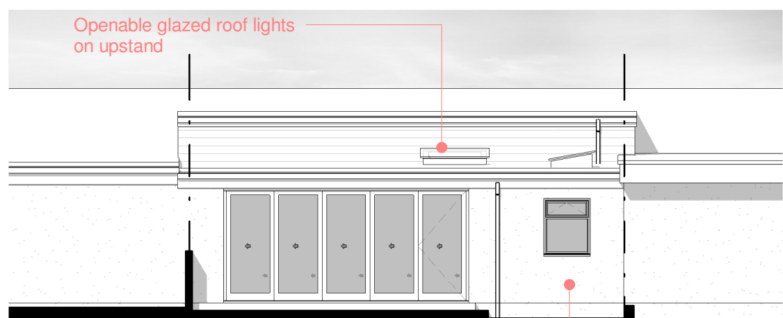
PROPOSED REAR 1 : 100
