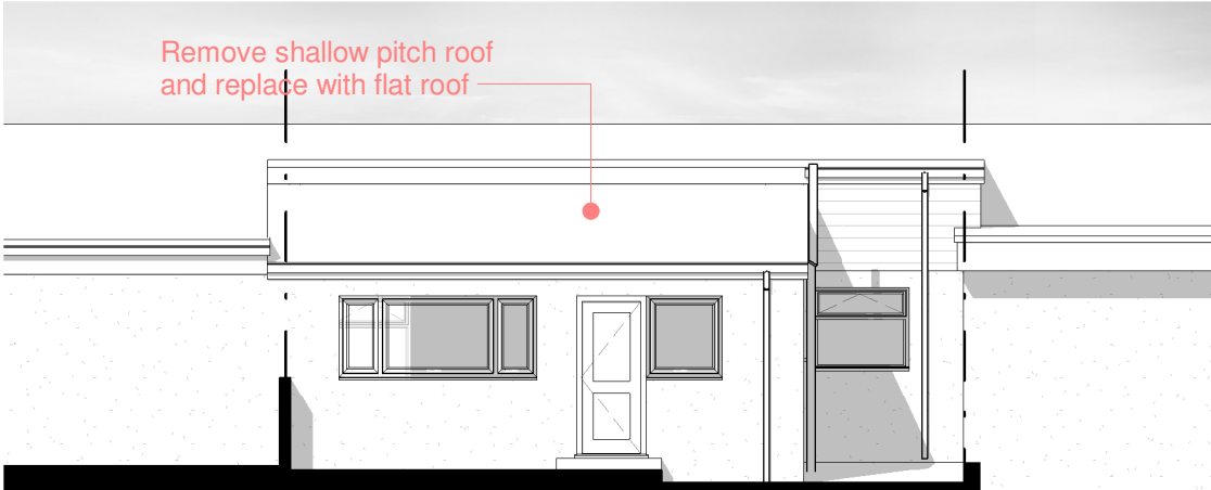
EXISTING REAR 1 : 100
