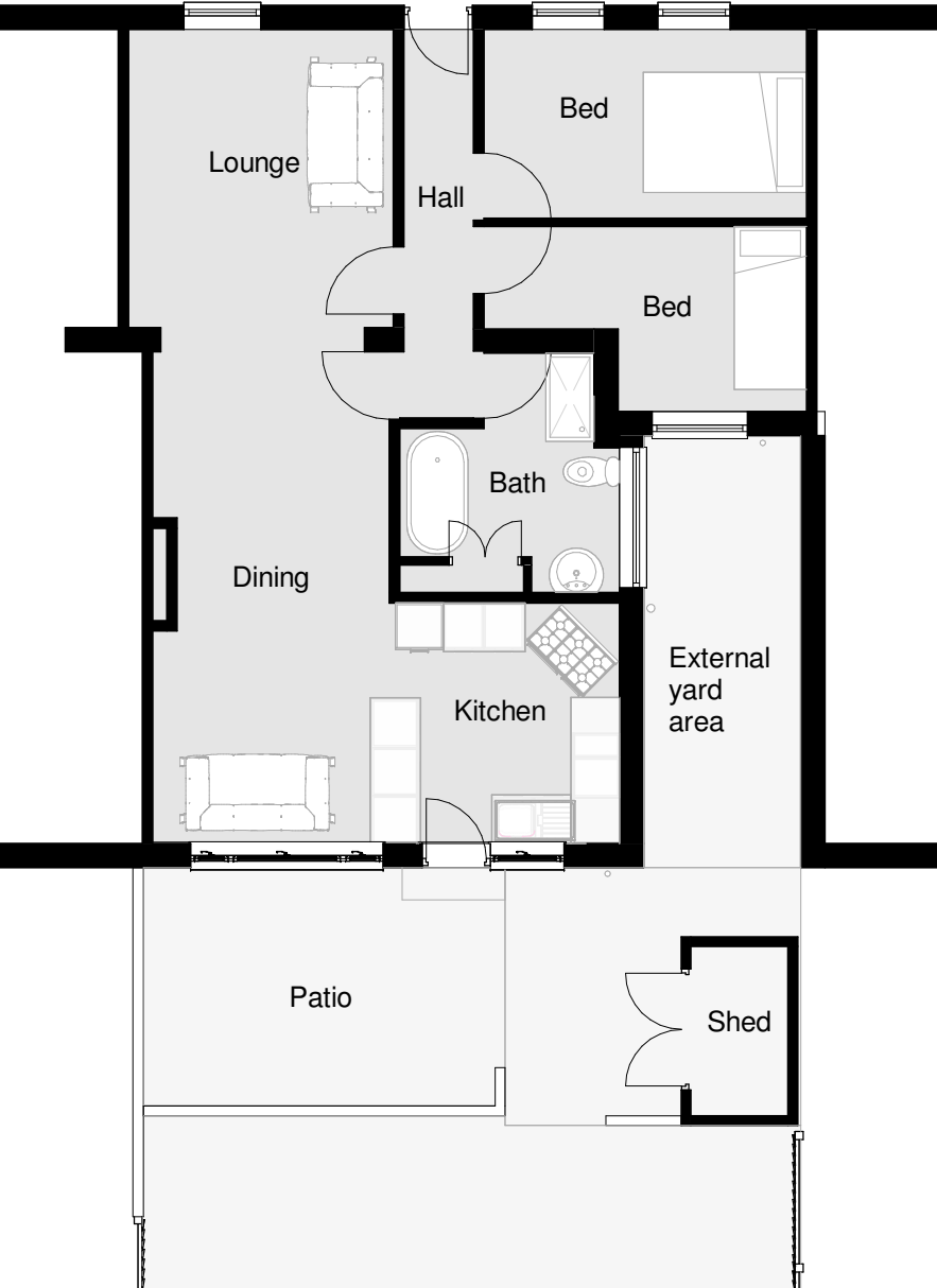
EXISTING FLOOR PLAN 1 : 100
