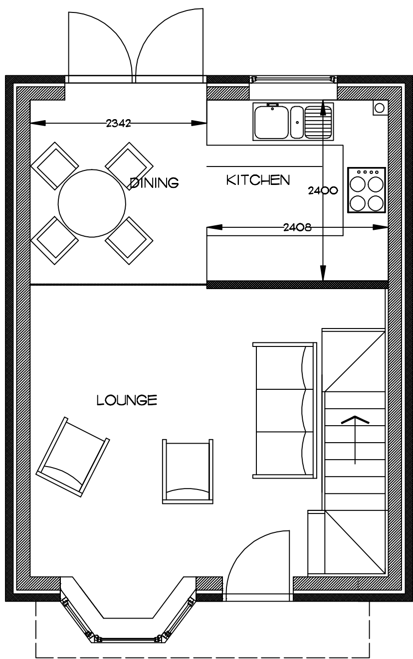
PROPOSED GROUND FLOOR PLAN PLOT 3 ONLY 1/50
