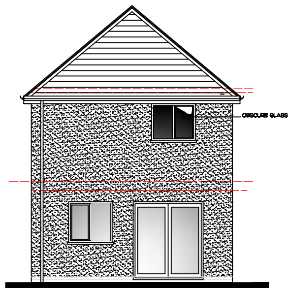
PROPOSED REAR ELEVATION PLOT 3 ONLY 1/100
