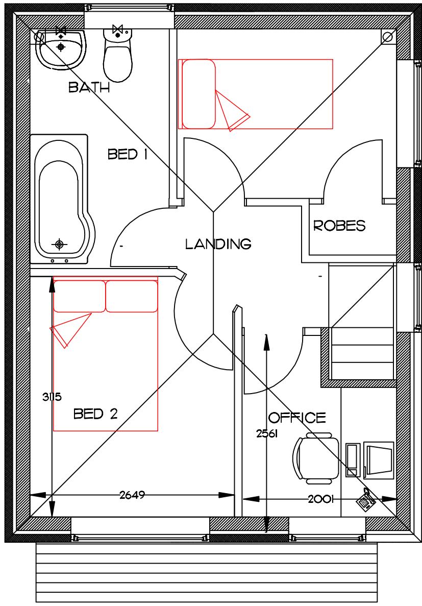
PROPOSED FIRST FLOOR PLAN PLOT 3 ONLY 1/50
