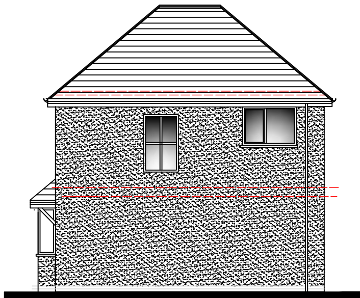
PROPOSED SIDE ELEVATION PLOTS 3 ONLY 1/100
