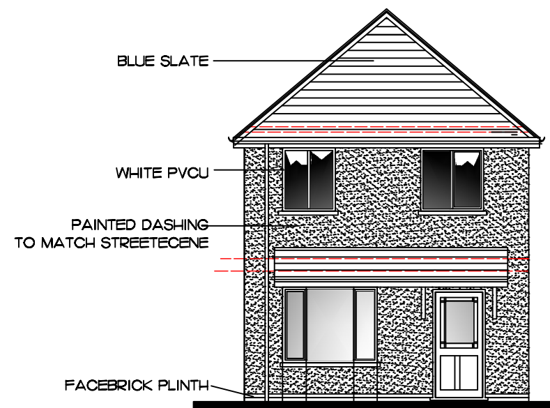
PROPOSED FRONT ELEVATION PLOT 3 ONLY 1/100
