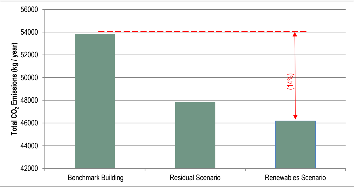
Figure E1: Implementation of the Energy Hierarchy for proposed Aldi development at Abbey Road, Neath.
