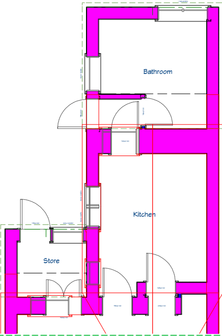
Existing and proposed floor plans
