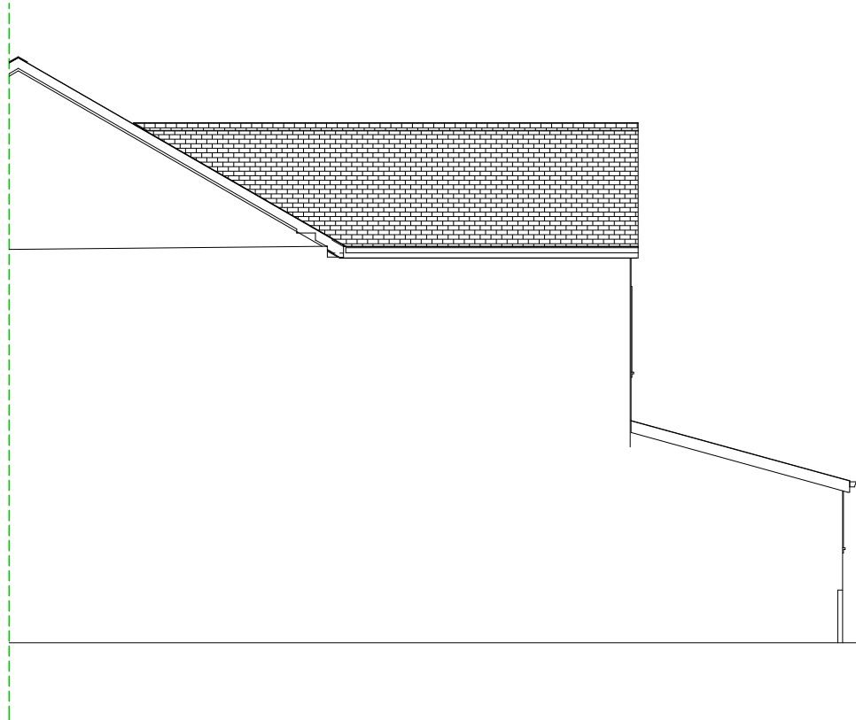
Existing second side elevation
