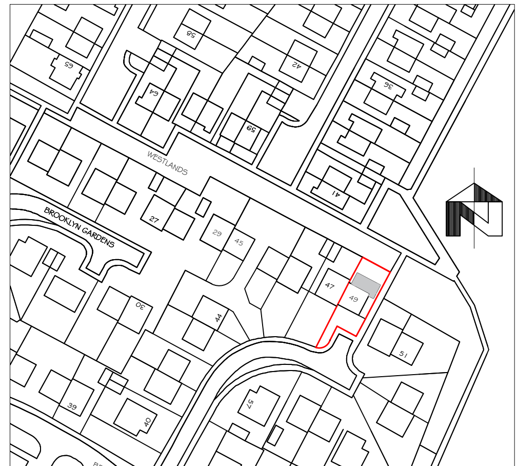
LOCATION PLAN 1:1250
