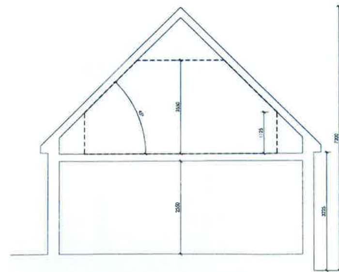
CROSS SECTION PROPOSED
