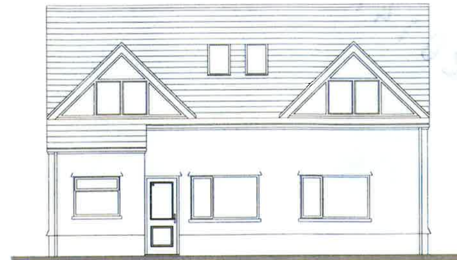
REAR ELEVATION PROPOSED
