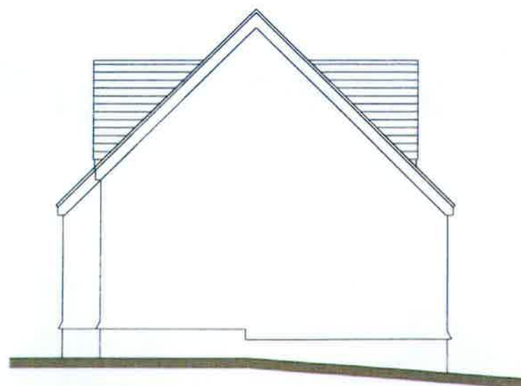
LEFT SIDE ELEVATION PROPOSED
