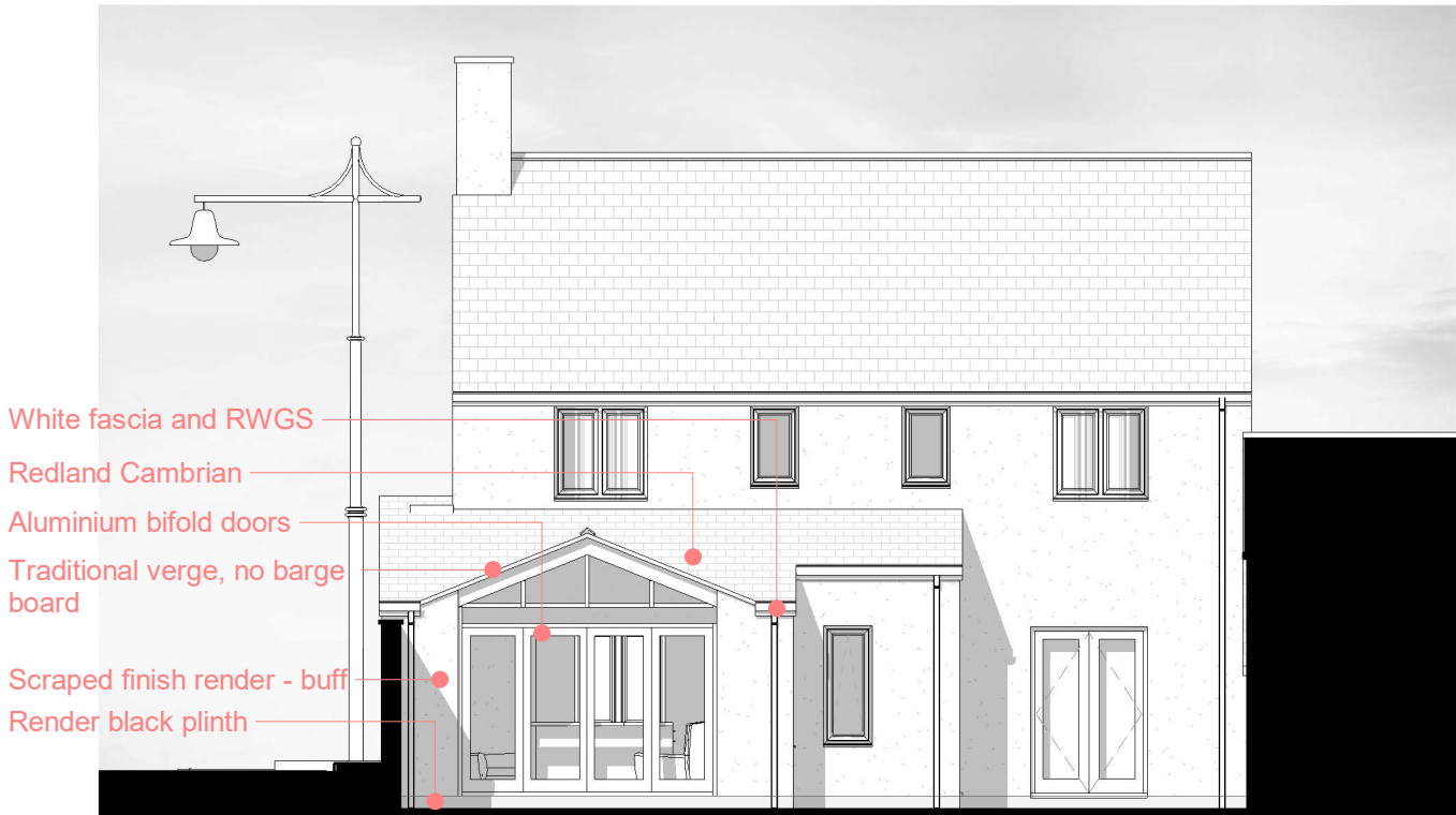
REAR ELEVATION (PROP) 1 : 100
