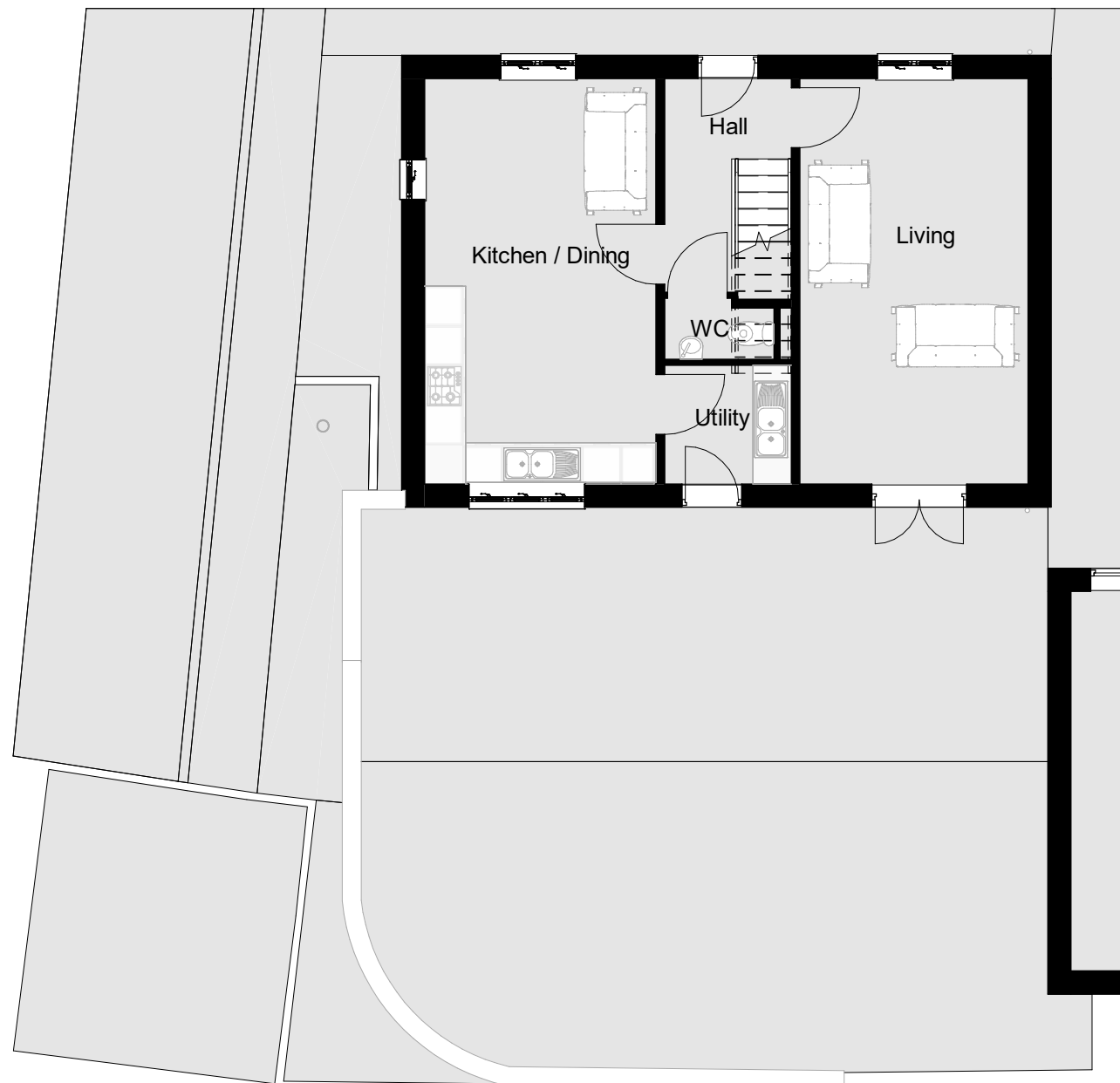
GROUND FLOOR (EXTG) 1 : 100
