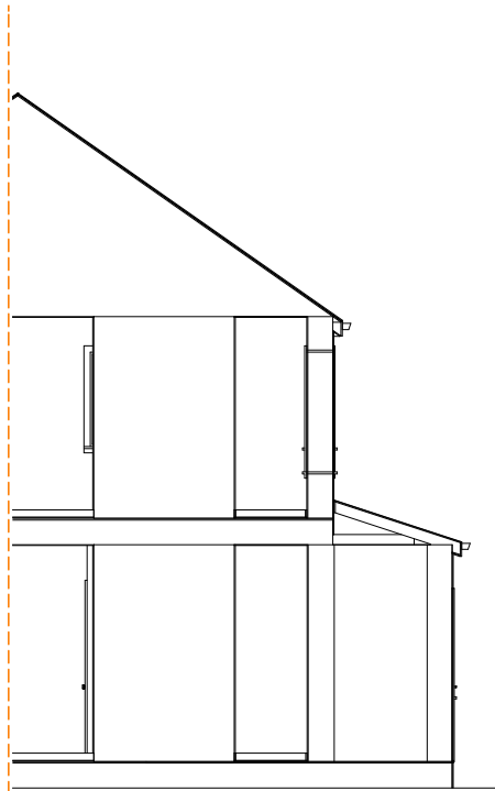
Existing second side elevation
