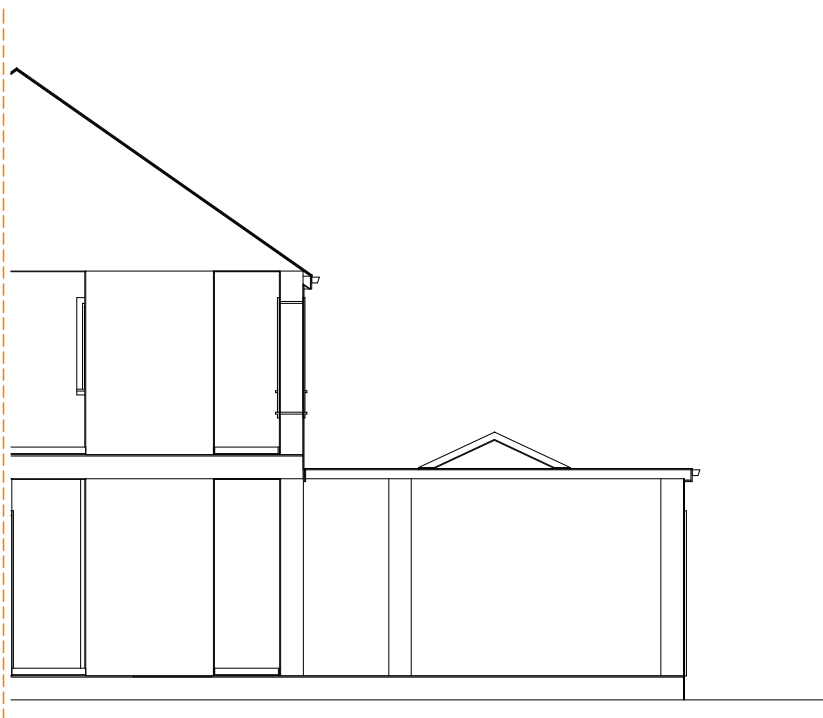
Proposed second side elevation
