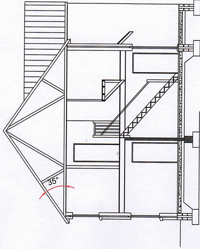
Section A 1:100
