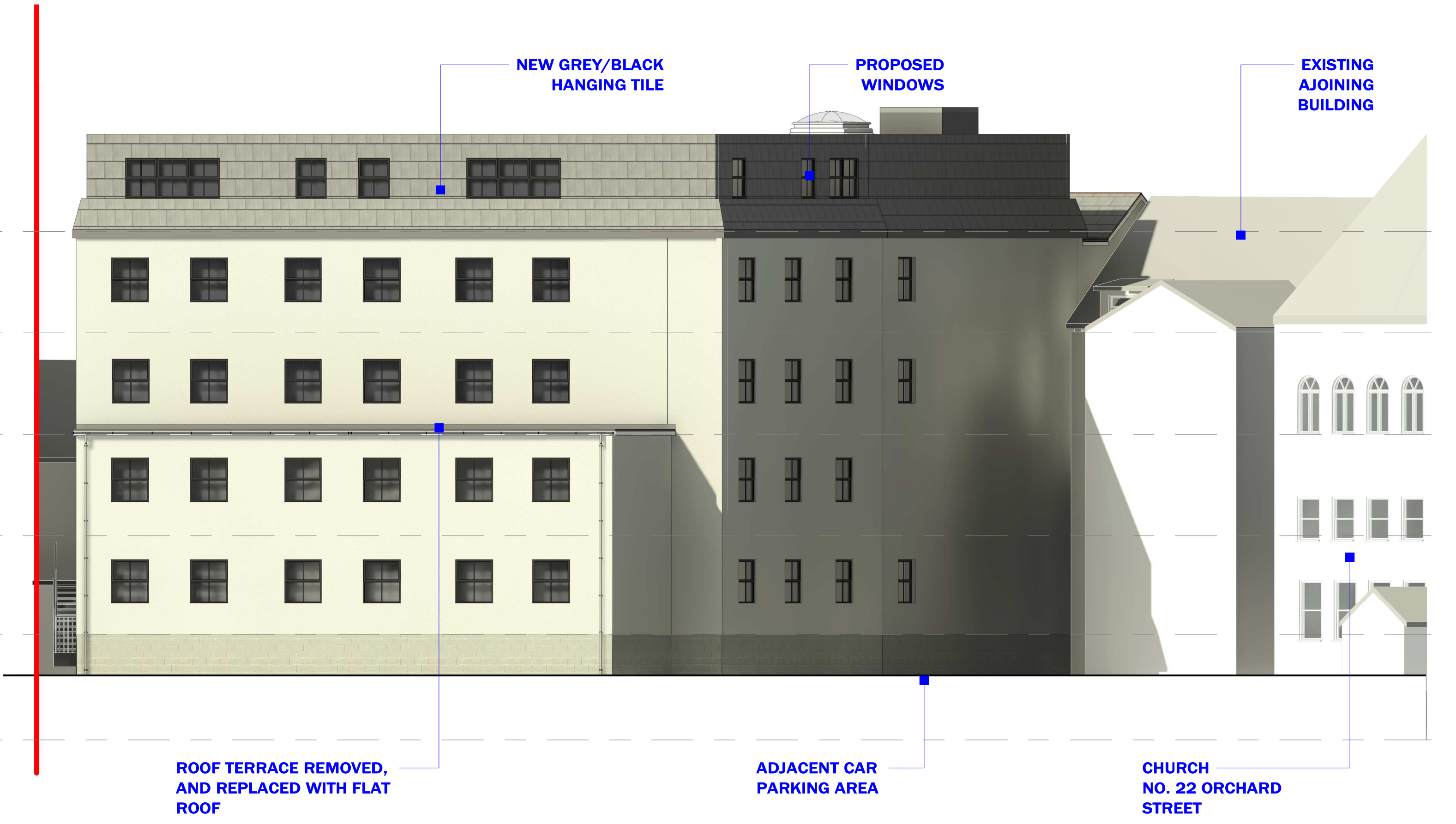
02 PROPOSED ELEVATION B 1 : 100
