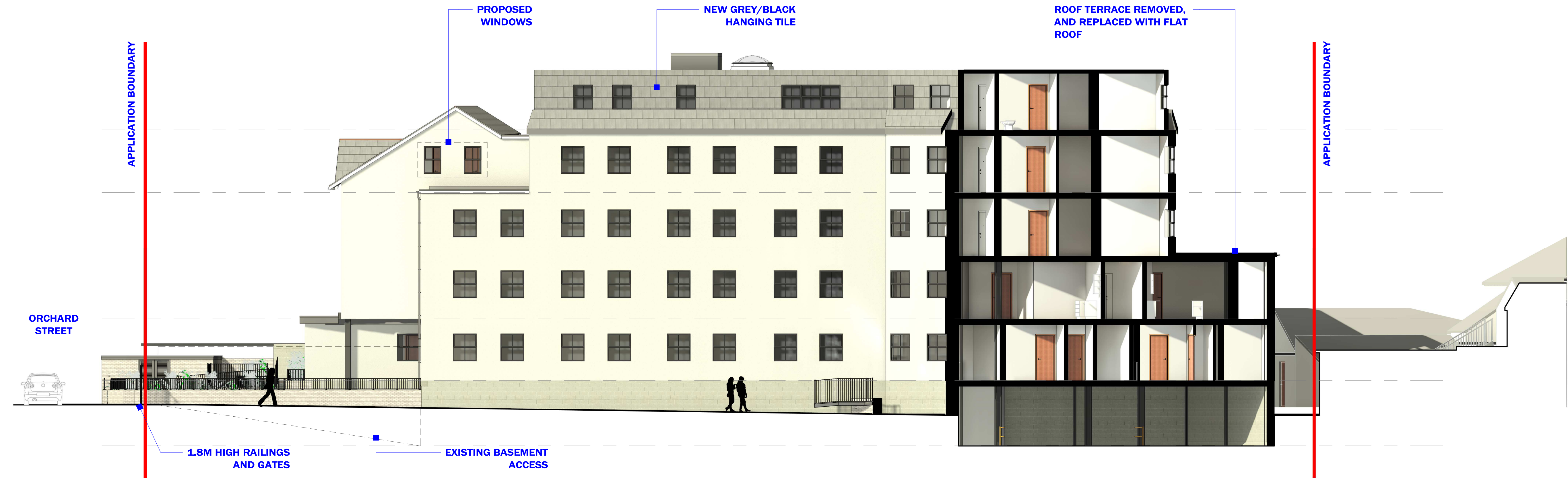
03 PROPOSED ELEVATION C 1 : 100
