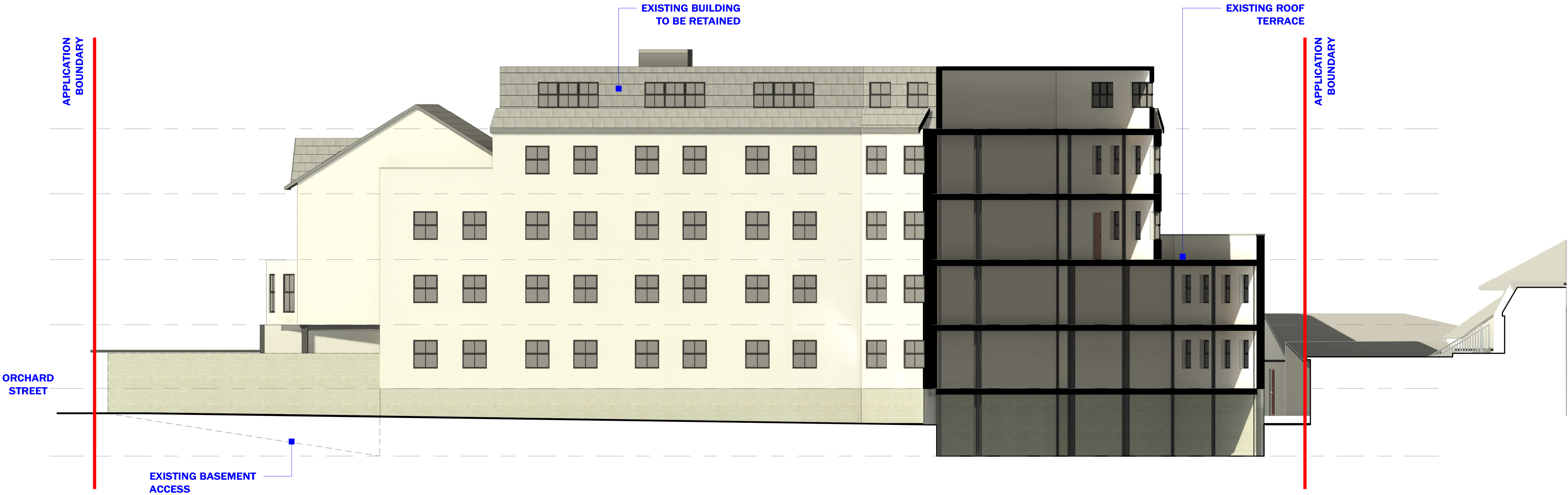
02 EXISTING ELEVATION C 1 : 100
