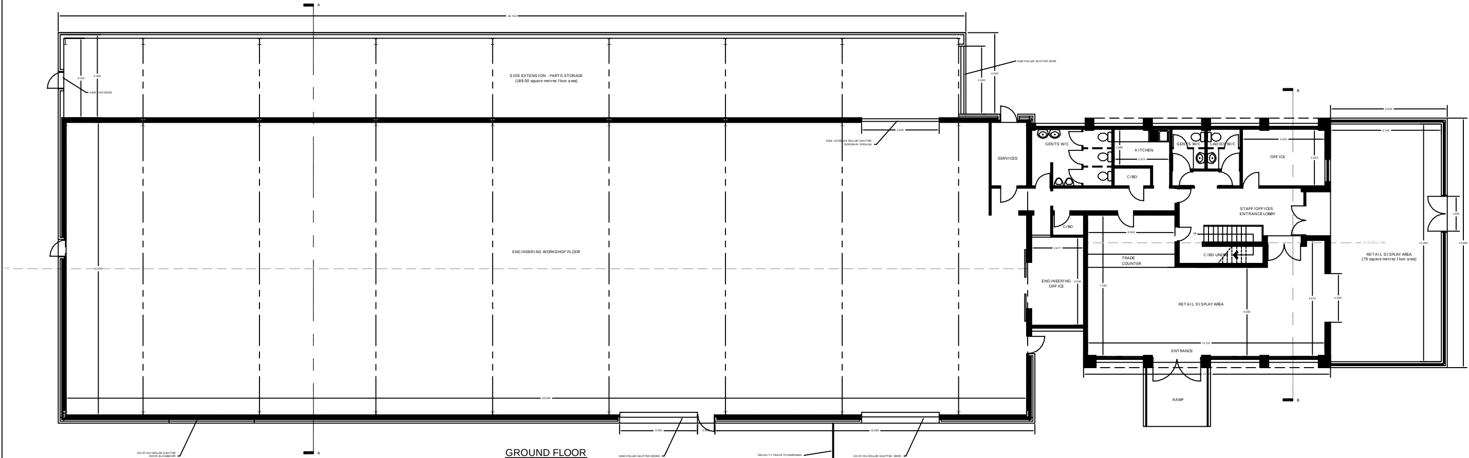
GROUND FLOOR
