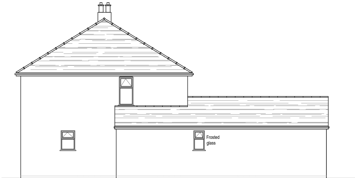
Proposed Elevation on 'A' scale - 1:100
