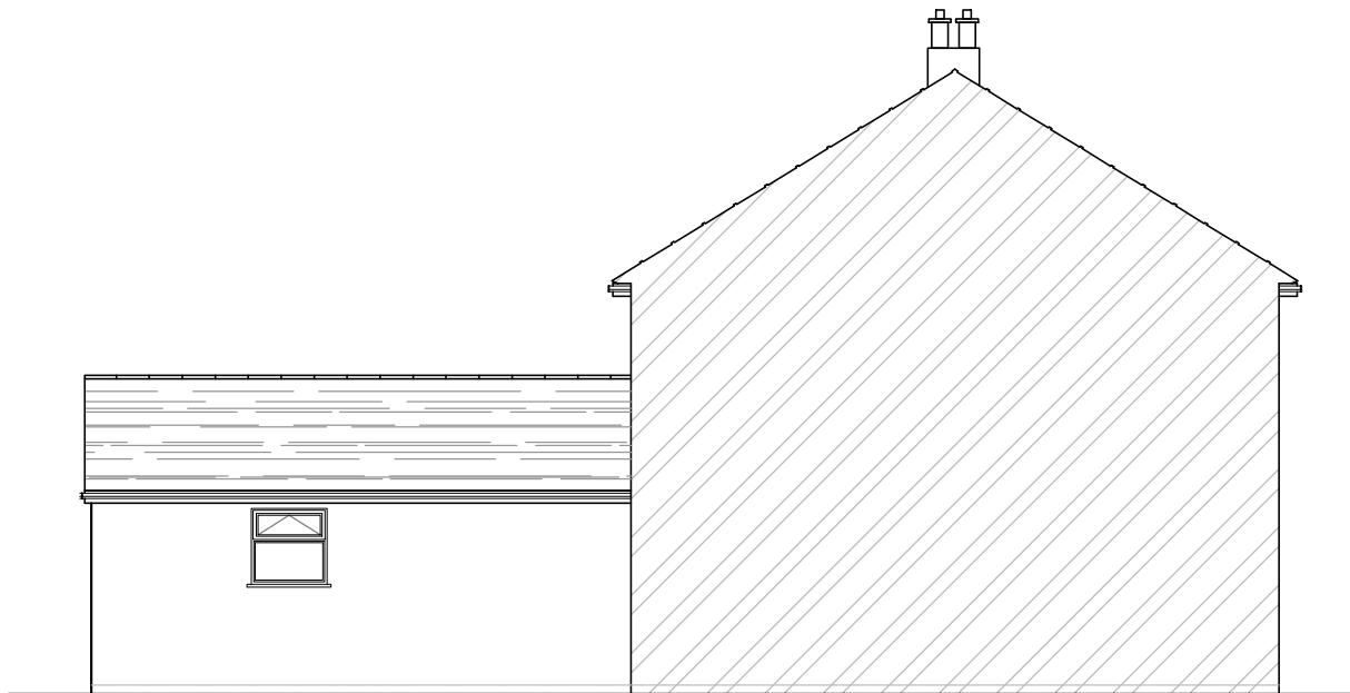
Proposed Elevation on 'B' scale - 1:100
