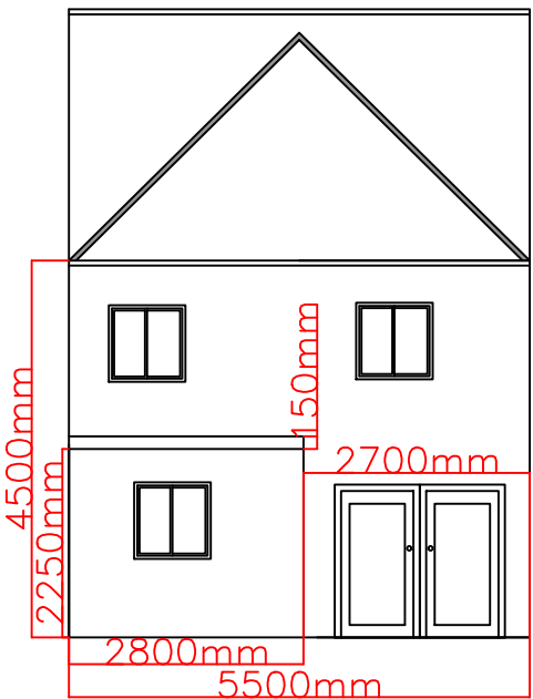
Rear Elevation View
