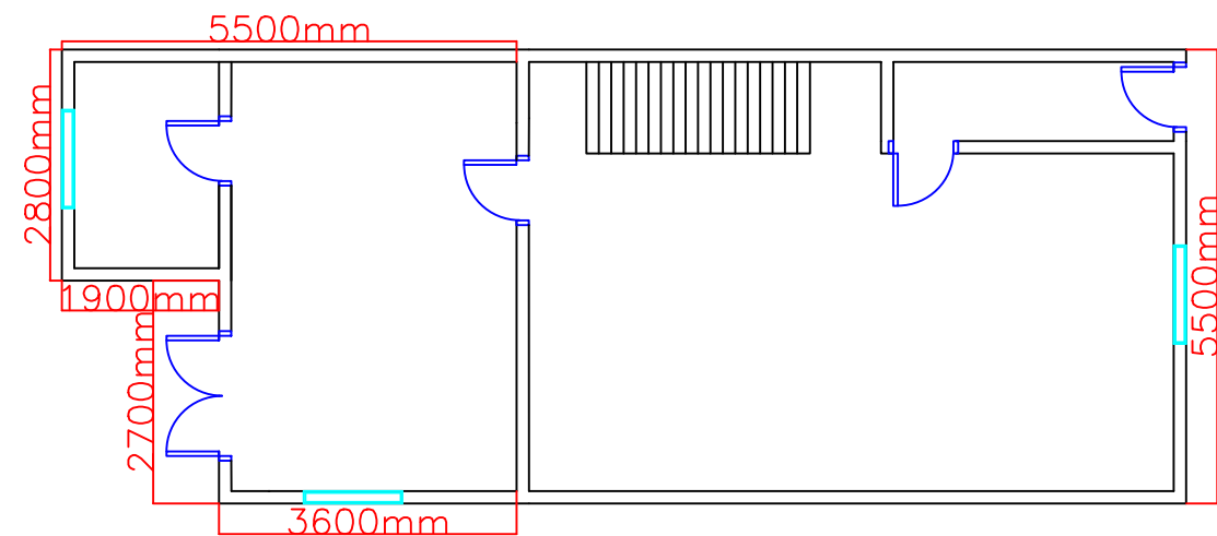
Proposed Floor Plan Ground Floor
