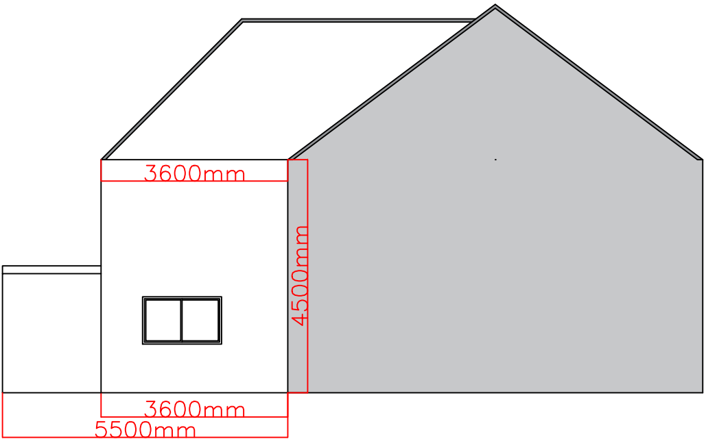
Side Elevation View
