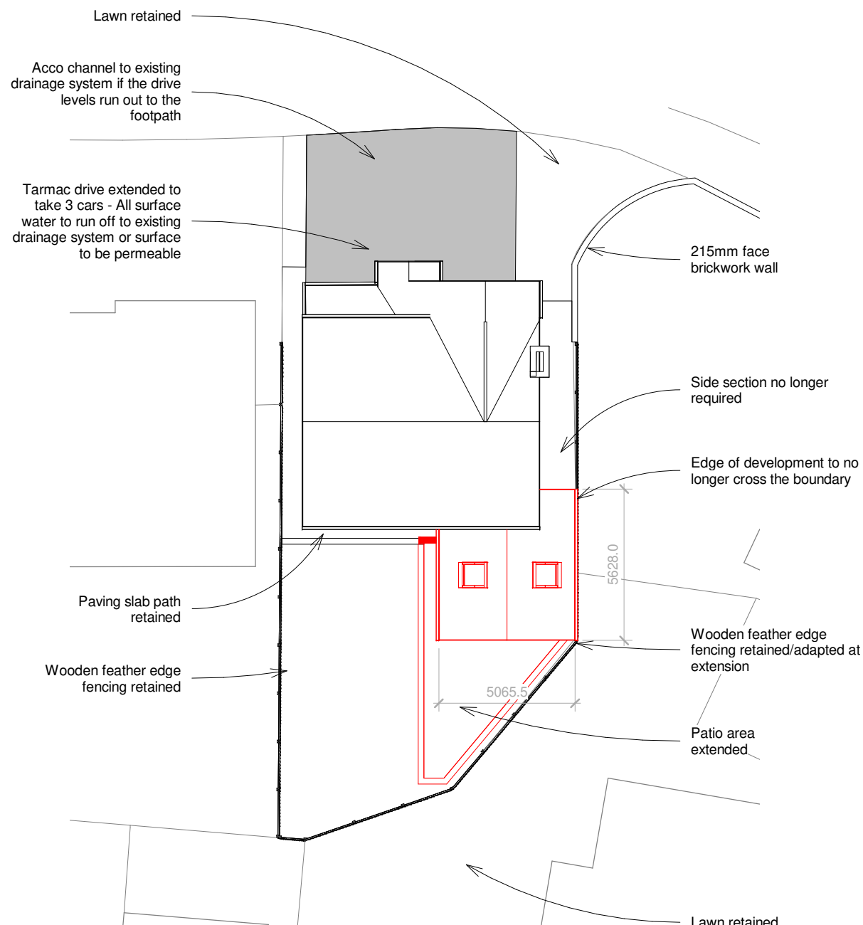
2 Site - Proposed 1 : 200
