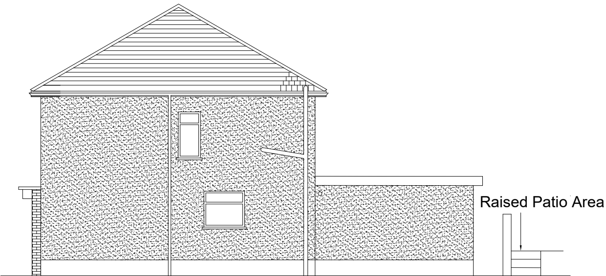
PROPOSED SIDE ELEVATION FACING NO22
