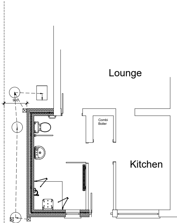
PROPOSED FLOOR LAYOUT
